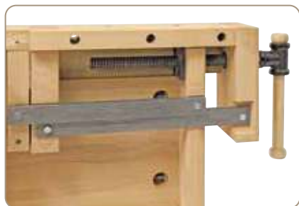
Prong bonded right clamping jaw with solid guide
