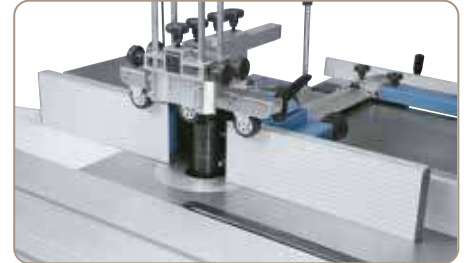
Solid moulding fence features fence rails with fine adjustment.
